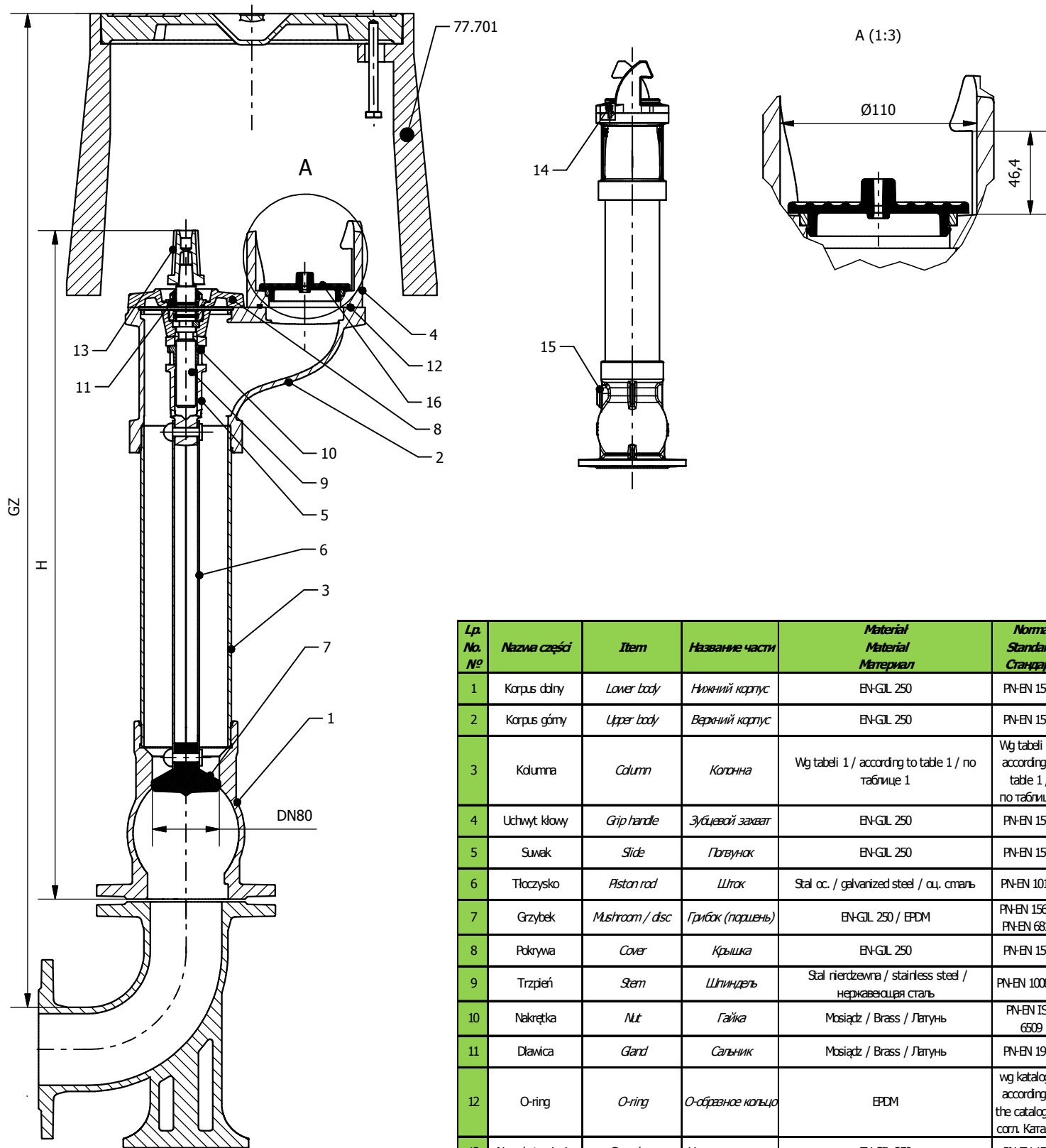
HP6 DN80 PN10 GJL 30.080.250.GZ.1
